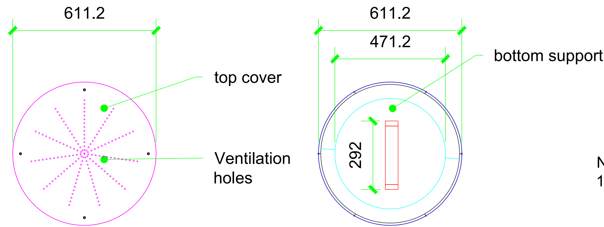
PLAN VIEW TOP VIEW
