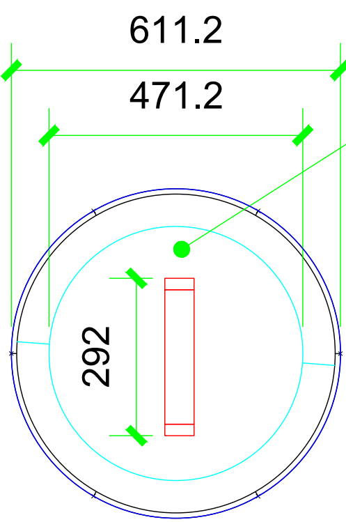
PLAN VIEW MIDDLE VIEW
