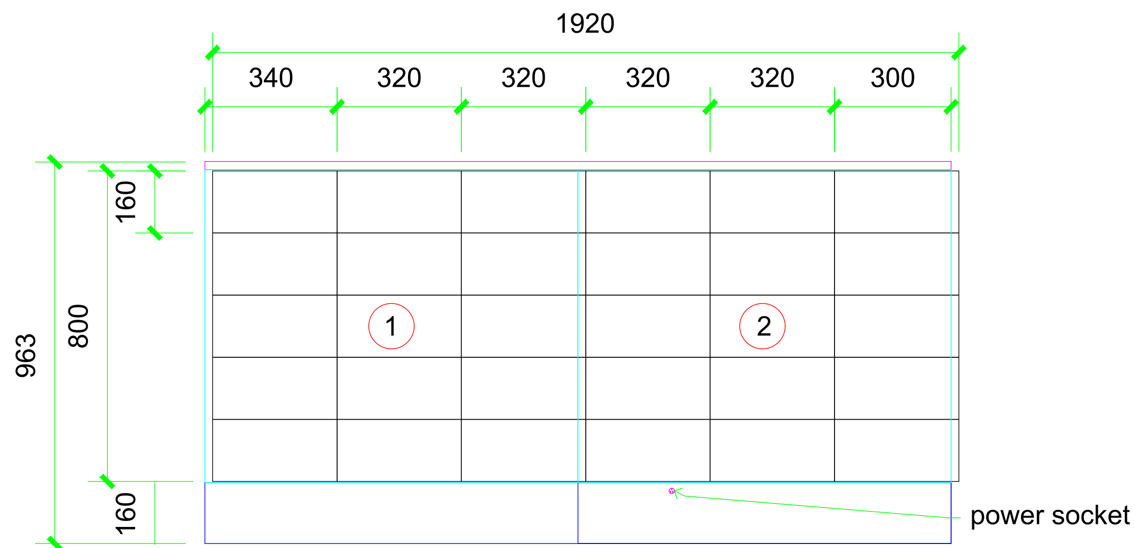
MODULE&CABINET FRONT UNFOLDED ARRAY FOR YOU INFORMATION ONLY,PLEASE CHECK THE PLAN VIEW
