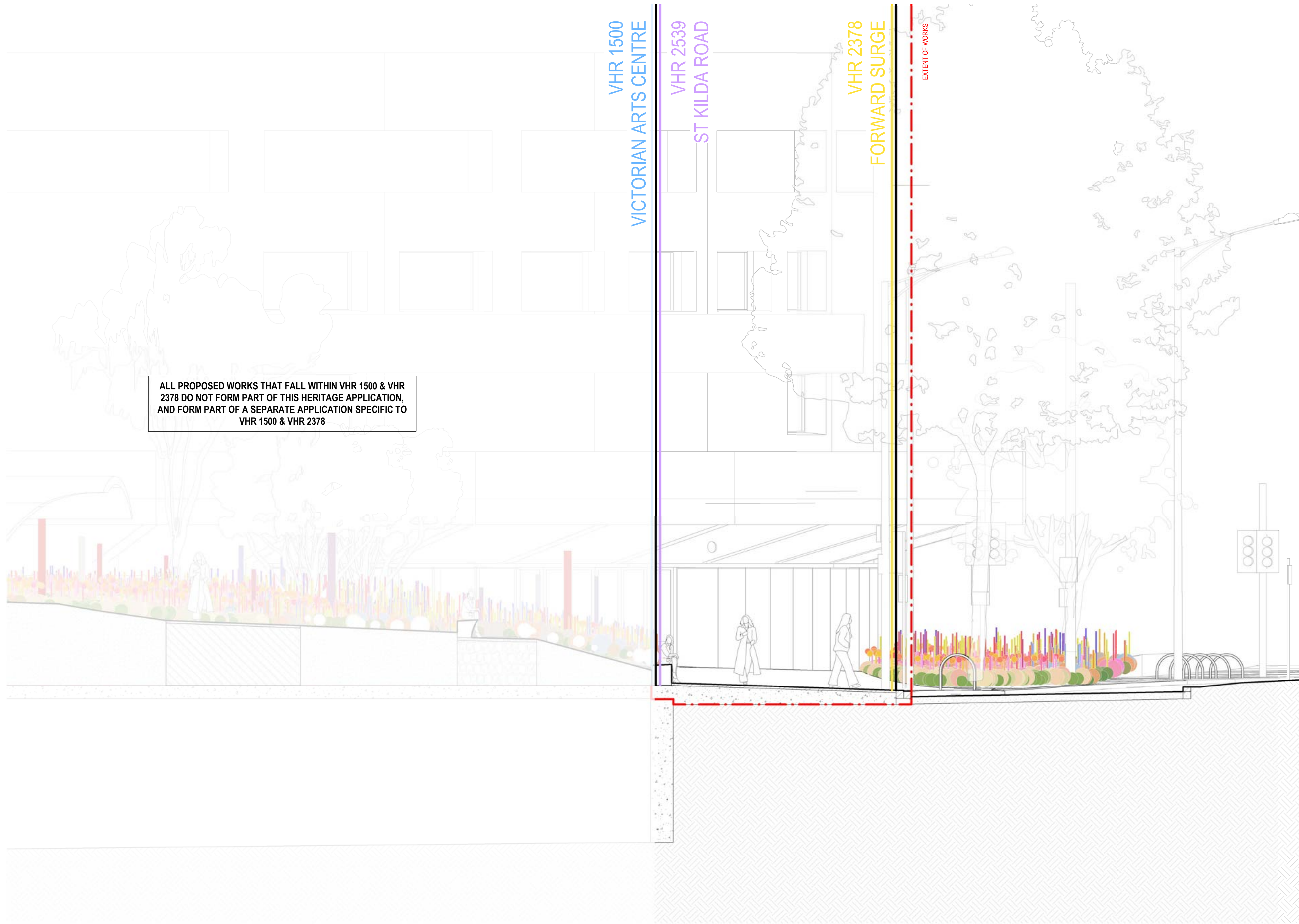
1 INTERFACE SECTION 04 1:50
