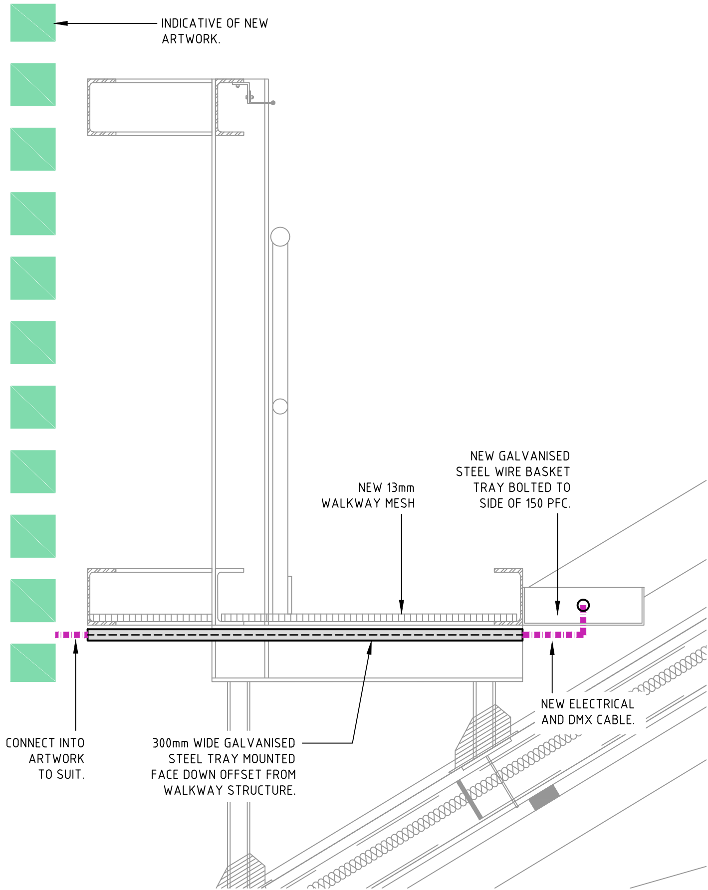
WALKWAY SECTION DETAIL SCALE 1:10 @ A1
