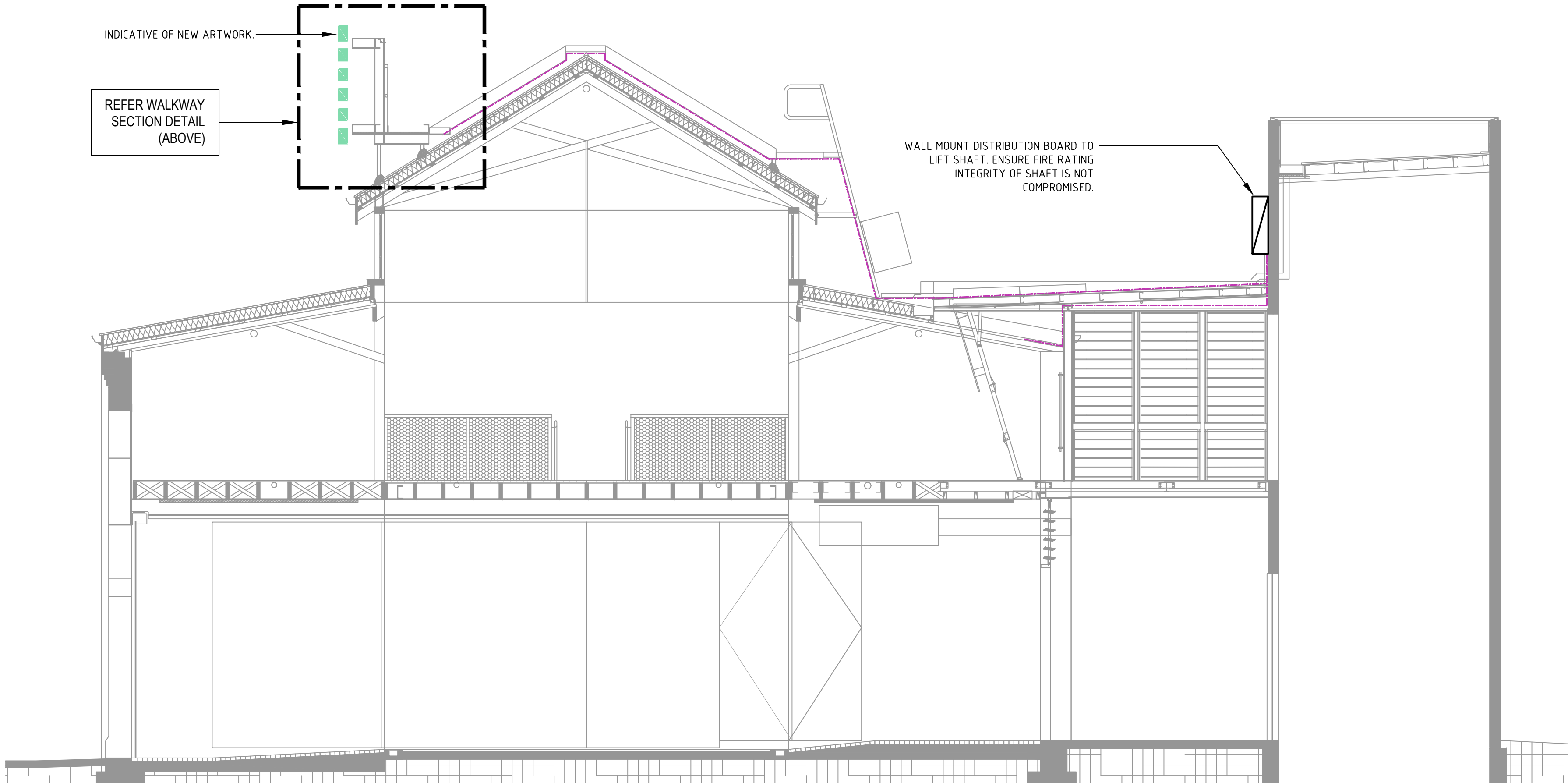
SECTION SCALE 1:50 @ A1
