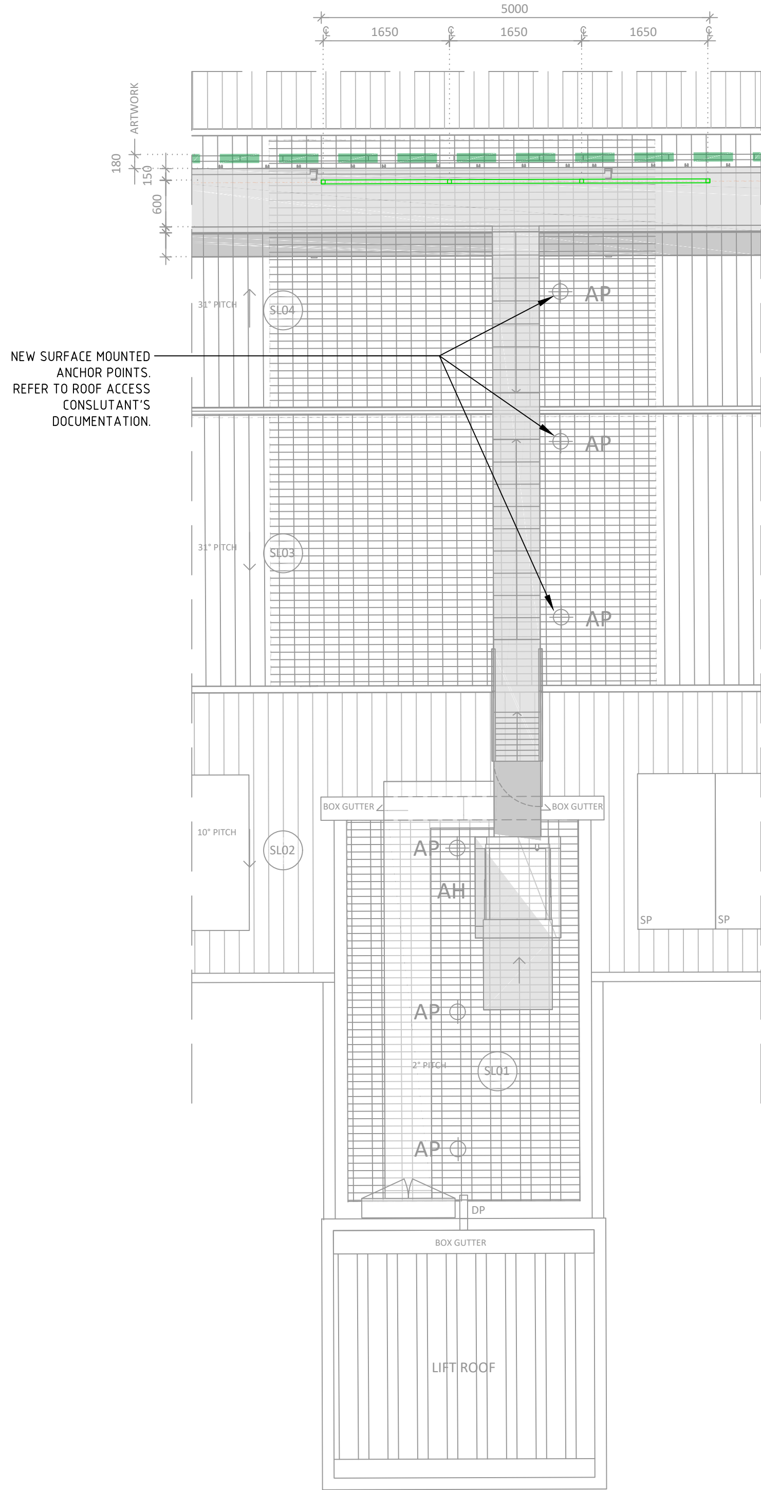
ROOF PLAN - ROOF ACCESS SCALE 1:50 @ A1
