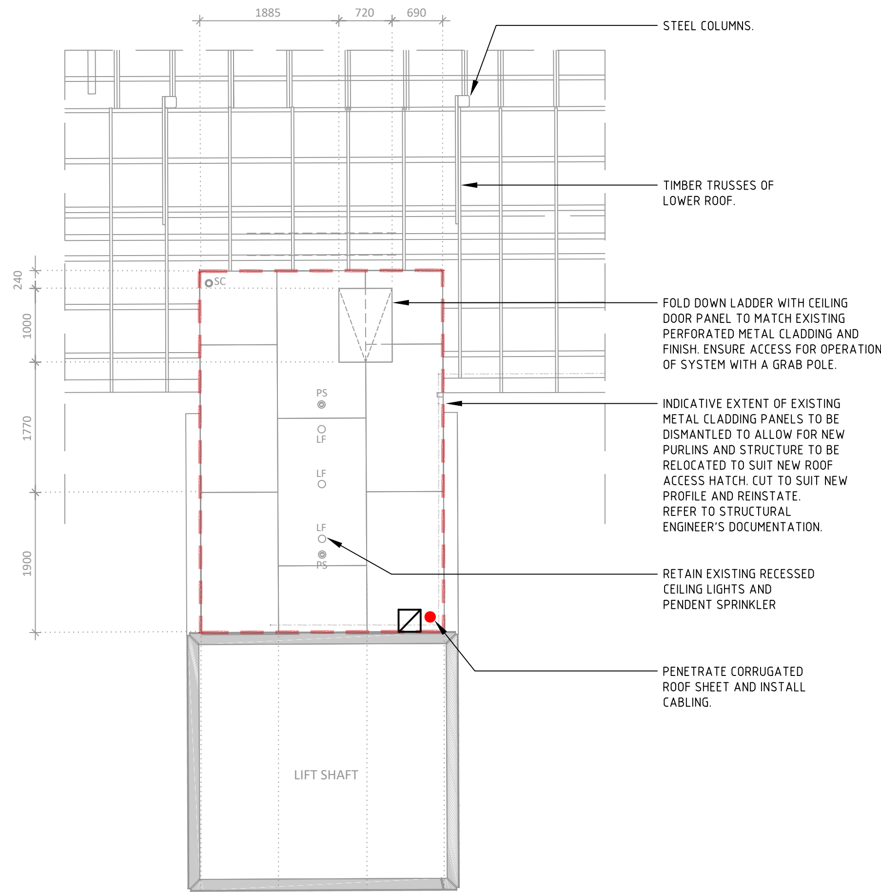
FIRST FLOOR REFLECTED CEILING PLAN SCALE 1:50 @ A1
