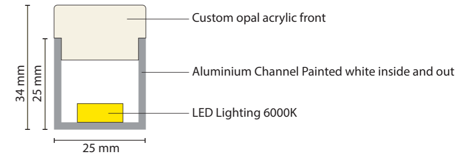
LED neon section detail
