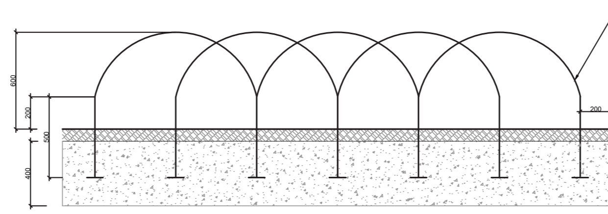
7 TYP. F1 - RE-BAR FENCING DETAIL
