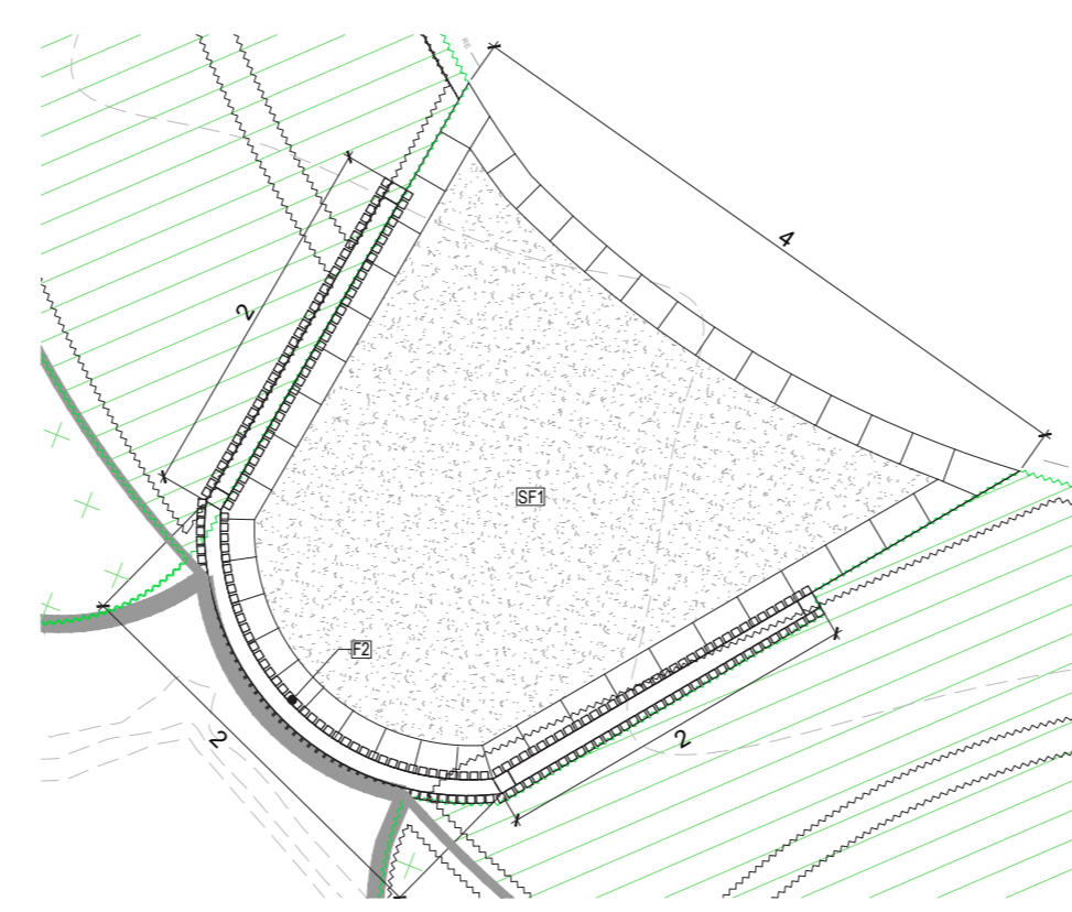
6 LANDING SETOUT PLAN
