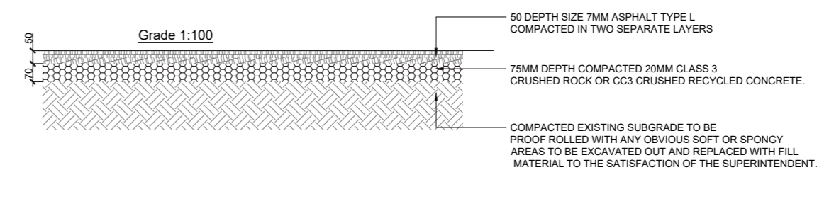
4 TYP. SF1 ASPHALT PAVEMENT DETAIL
