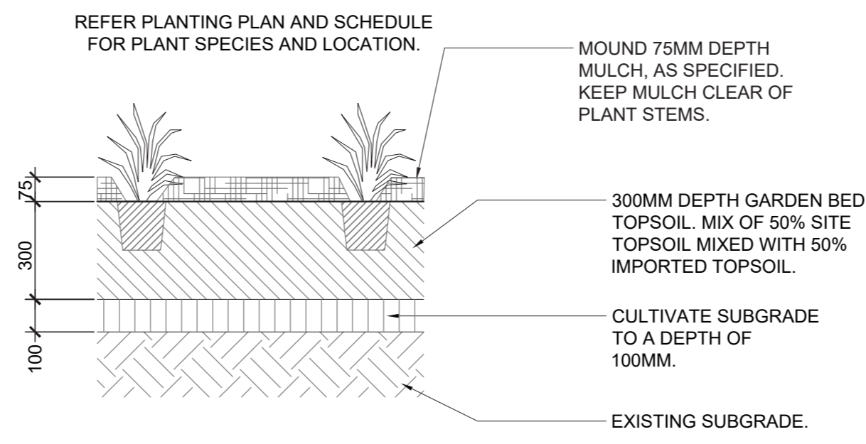
Garden Bed planting Detail
