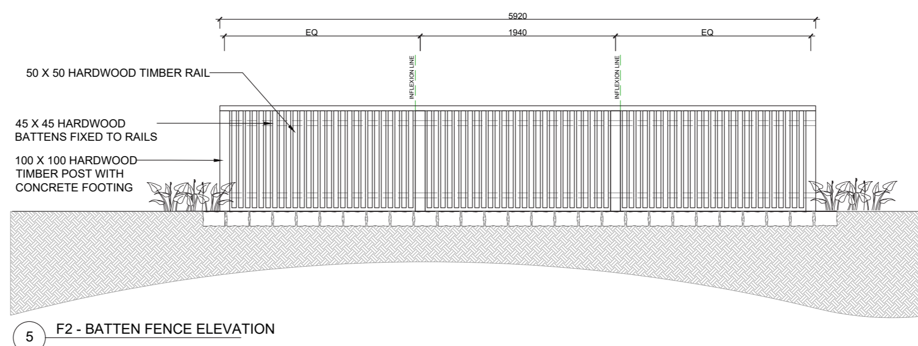
5 F2 - BATTEN FENCE ELEVATION
