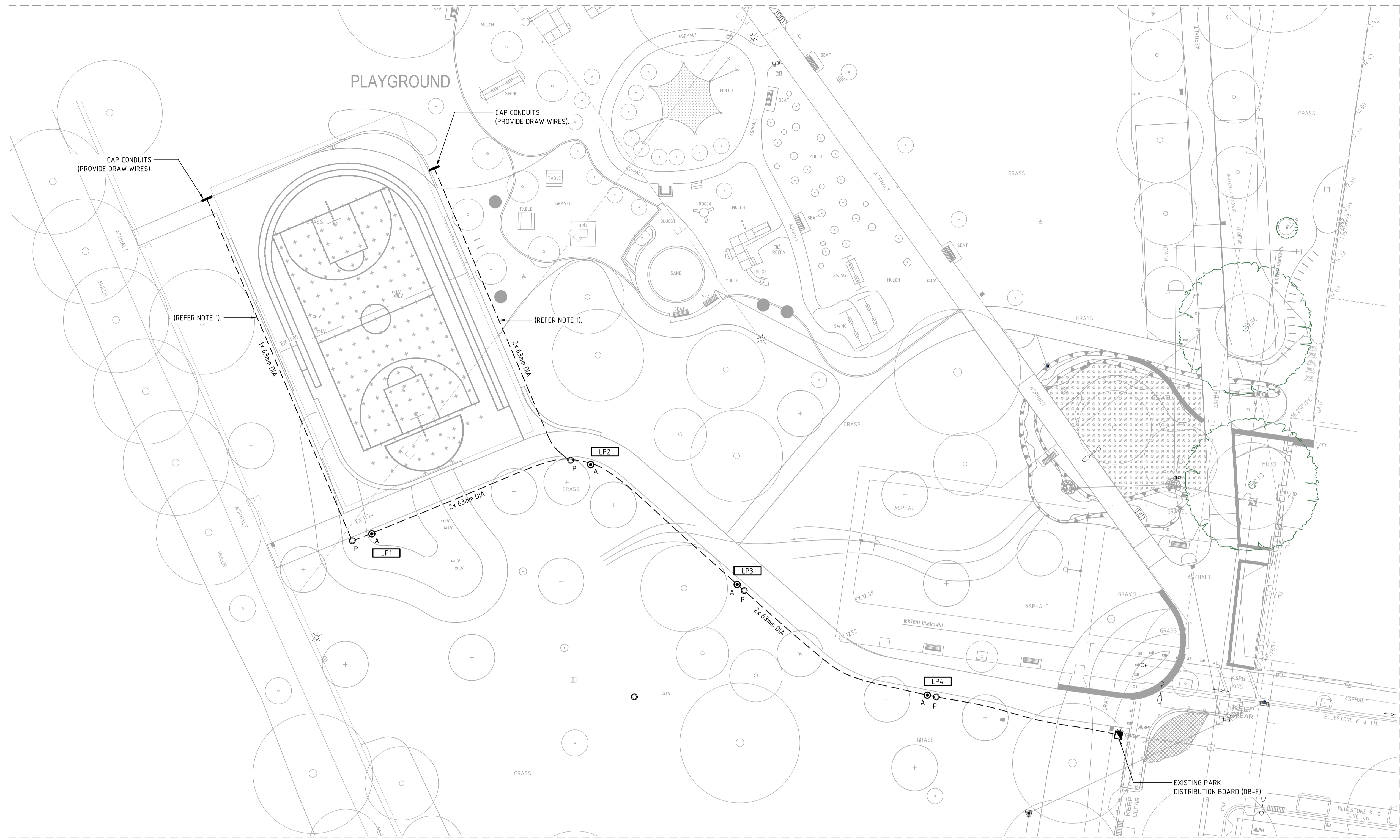
FAWKNER PARK - PAISLEY STREET NORTH SCALE 1:250 @ A1; 1:500 @ A3
