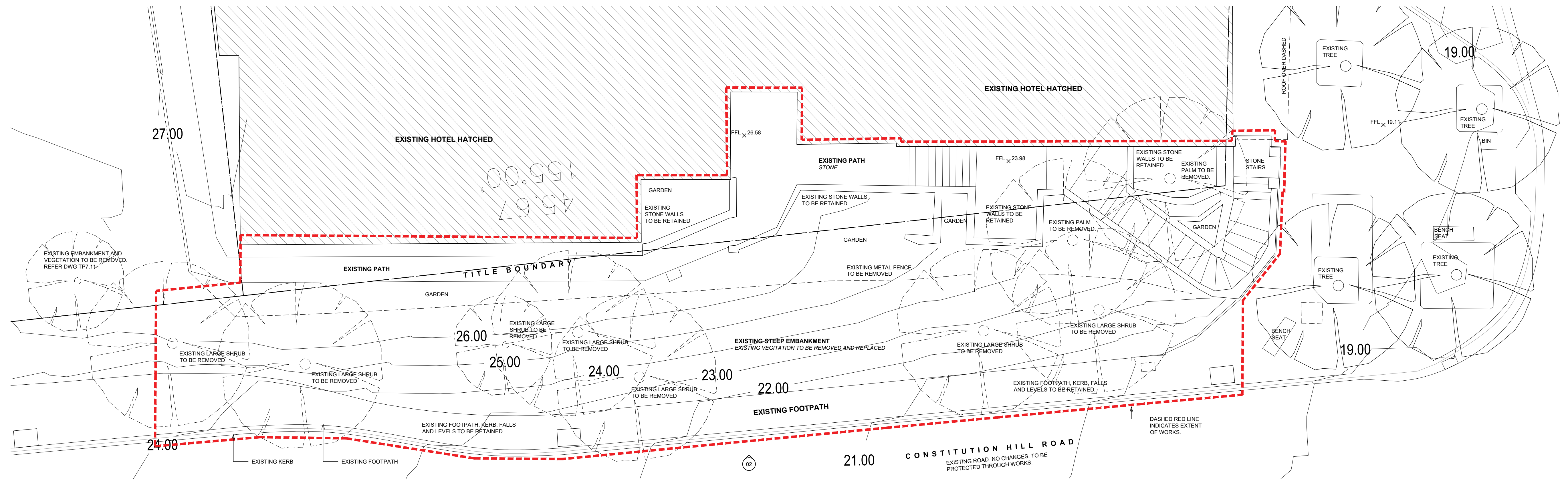
01 EXISTING PLAN - CONSTITUTION HILL ROAD LANDSCAPING 1:100
